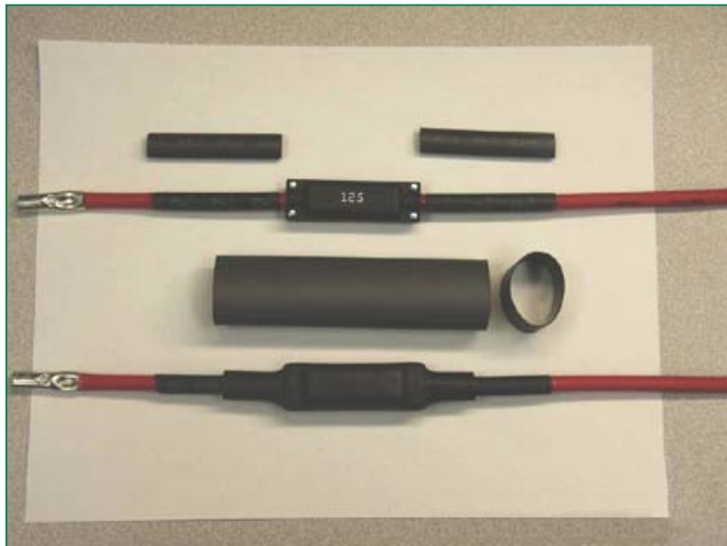
Example of the use of heat shrink tubing on CablePro® fuse.
