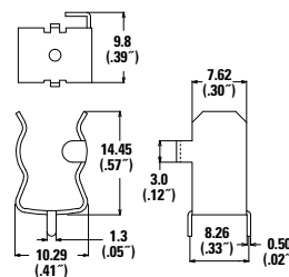
106 001 Device Dimensions
